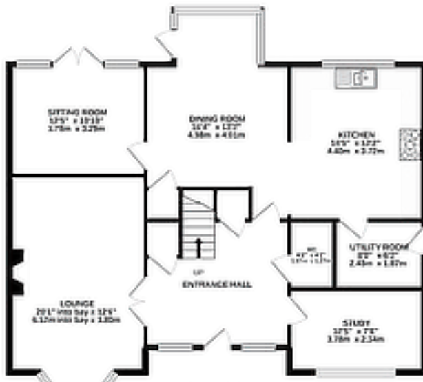
1ST FLOOR 1050 sq.ft. (97.6 sq.m.) approx.
